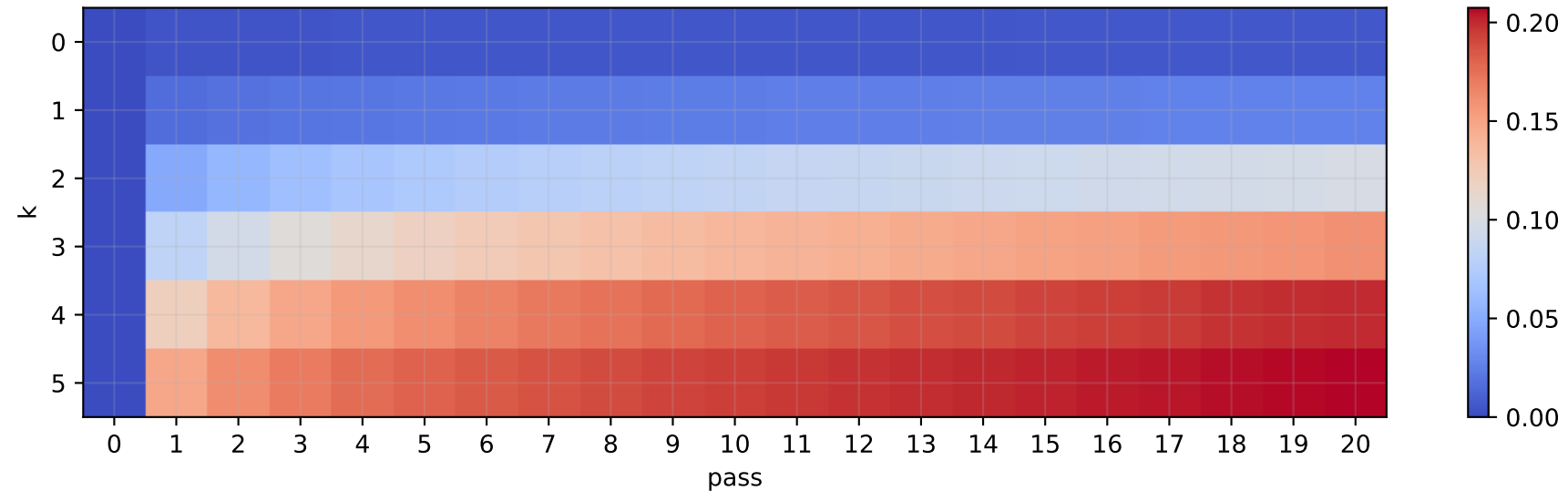
Covertime: Validation NLL - train NLL
