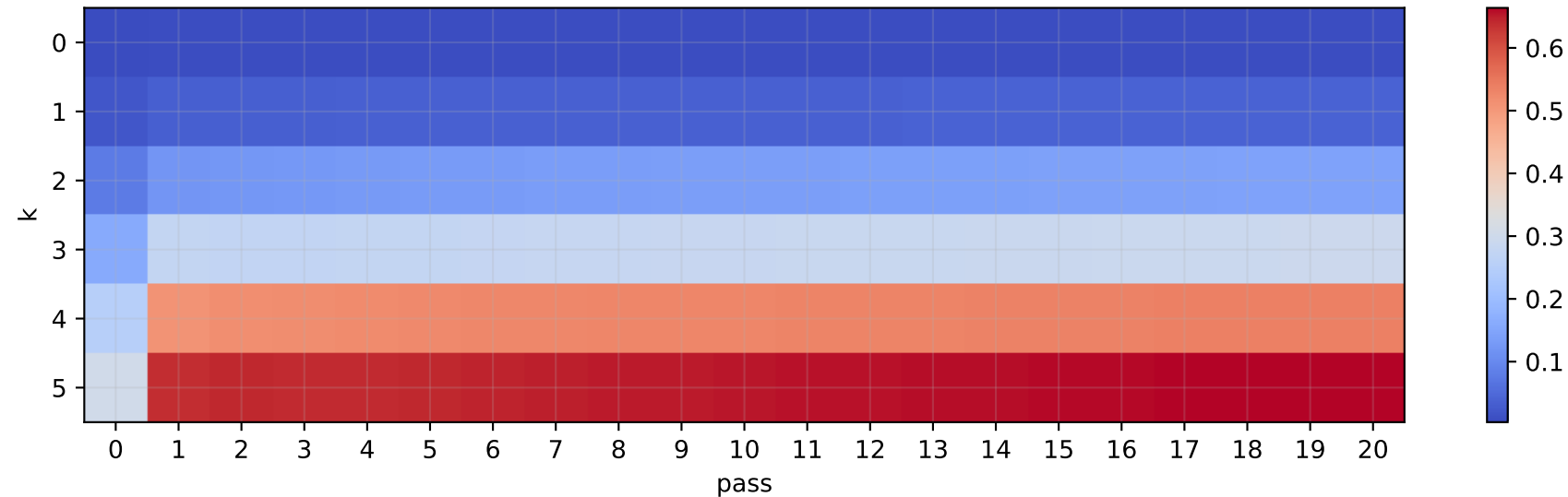
Covertypes: Validation NLL - train NLL
