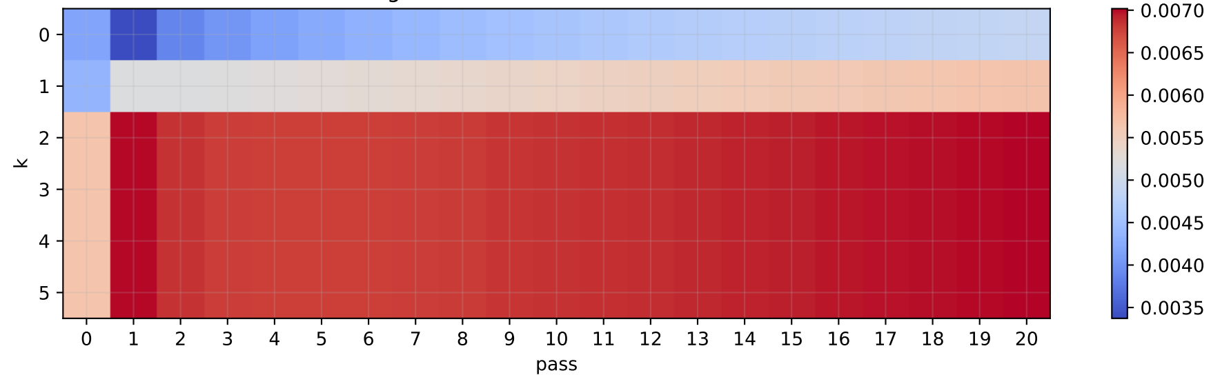
Skin Segmentation: Validation NLL - train NLL
