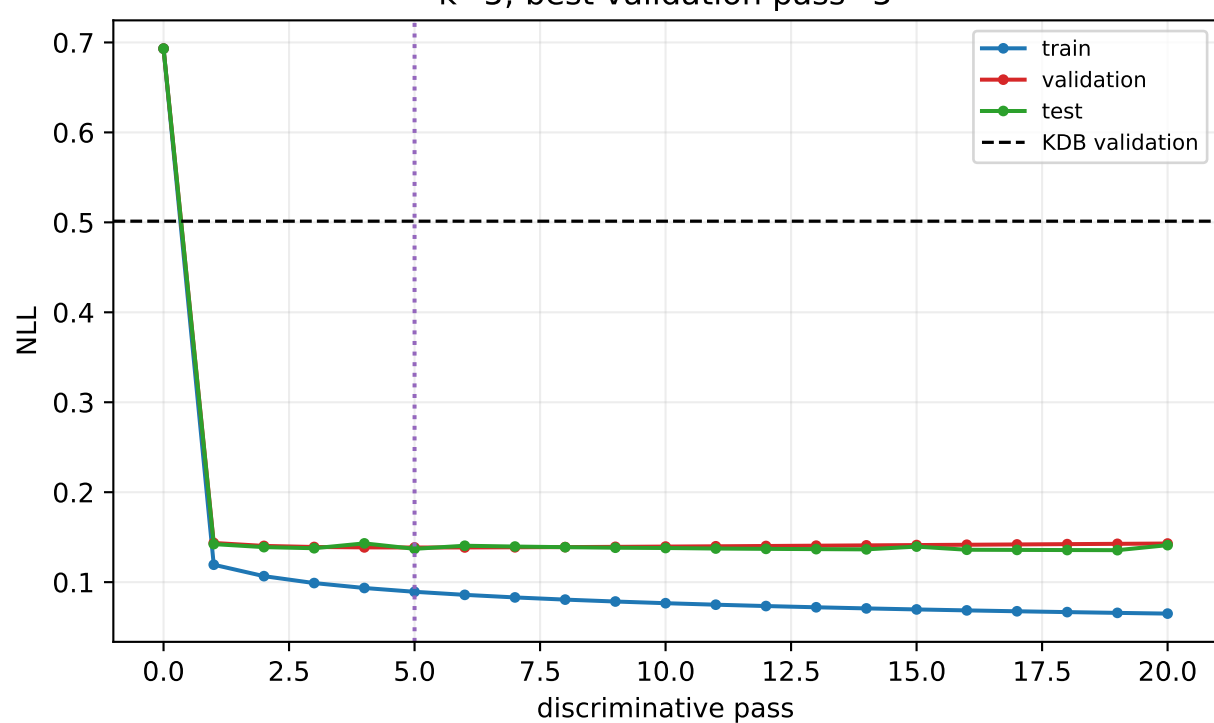
k=5; best validation pass=5
