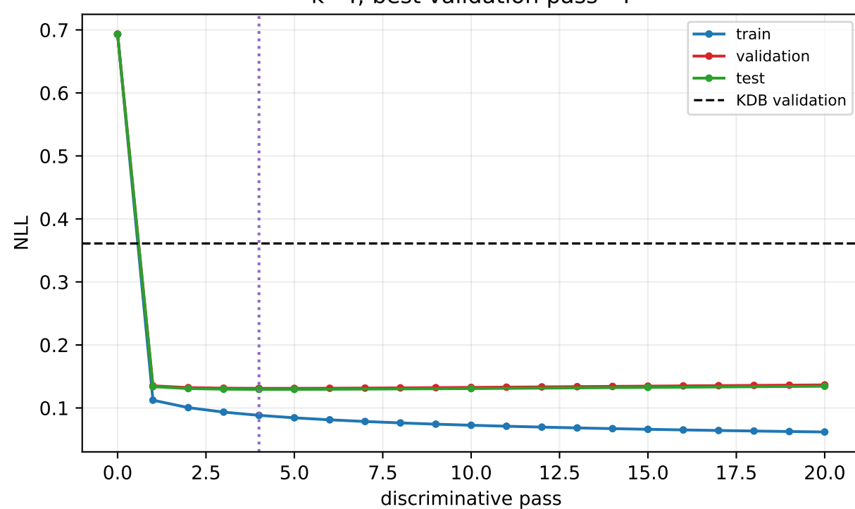
k=4; best validation pass=4
