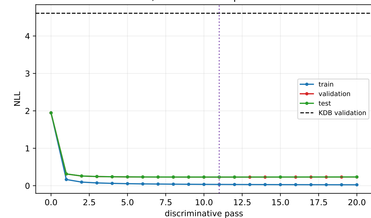
k=5; best validation pass=11
