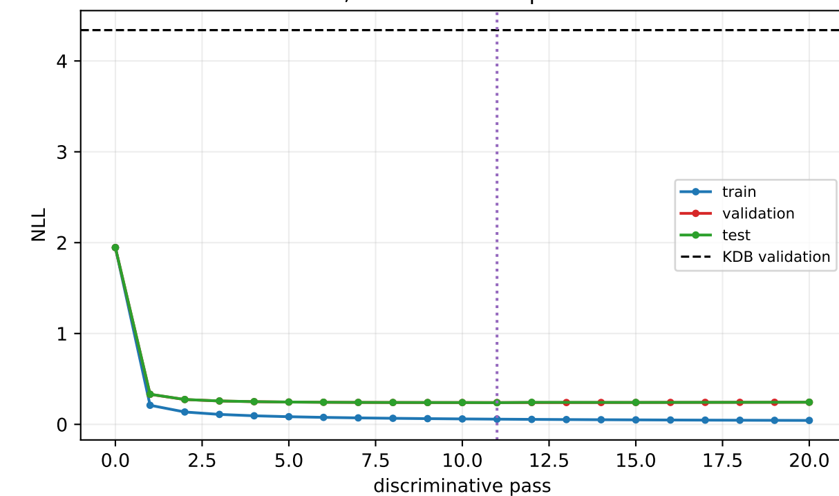
k=4; best validation pass=11
