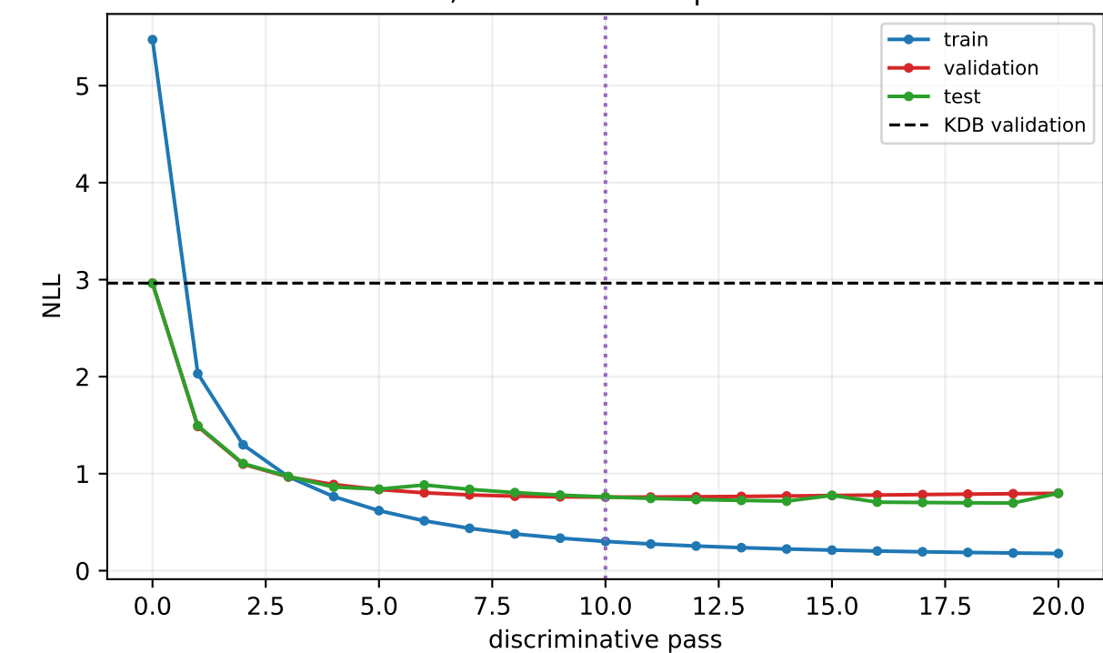
k=5; best validation pass=10
