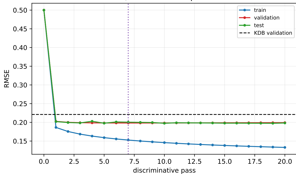
k=5; best validation pass=7
