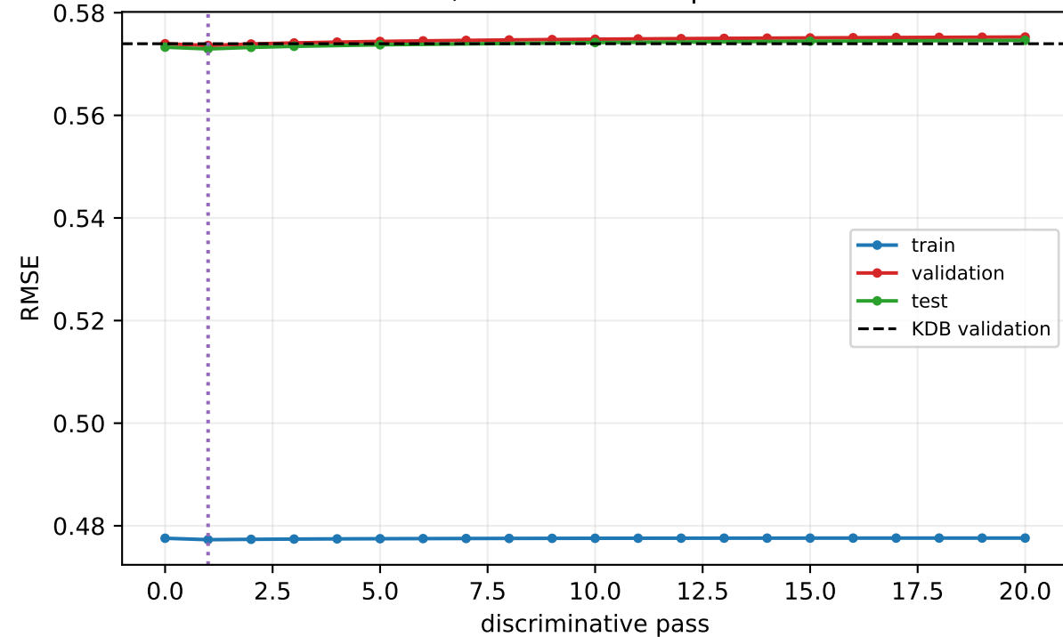
k=5; best validation pass=1
