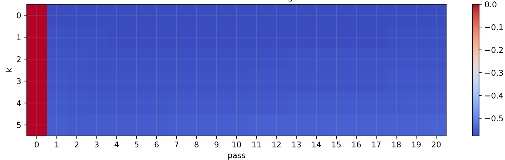
CensusIncome: Validation NLL change from initial
