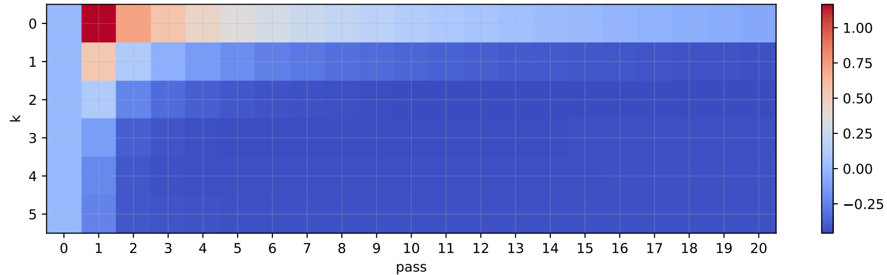
MiniBooNE: Validation NLL change from initial
