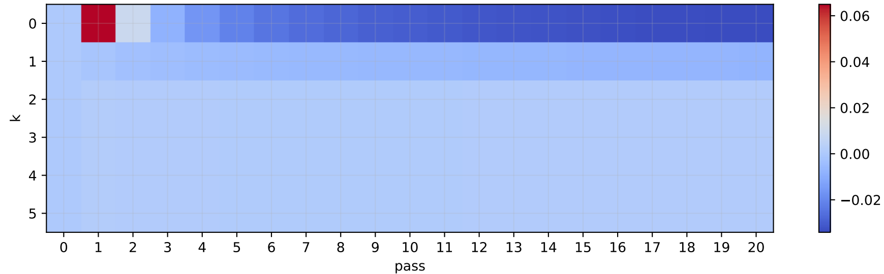
Skin Segmentation: Validation NLL change from initial
