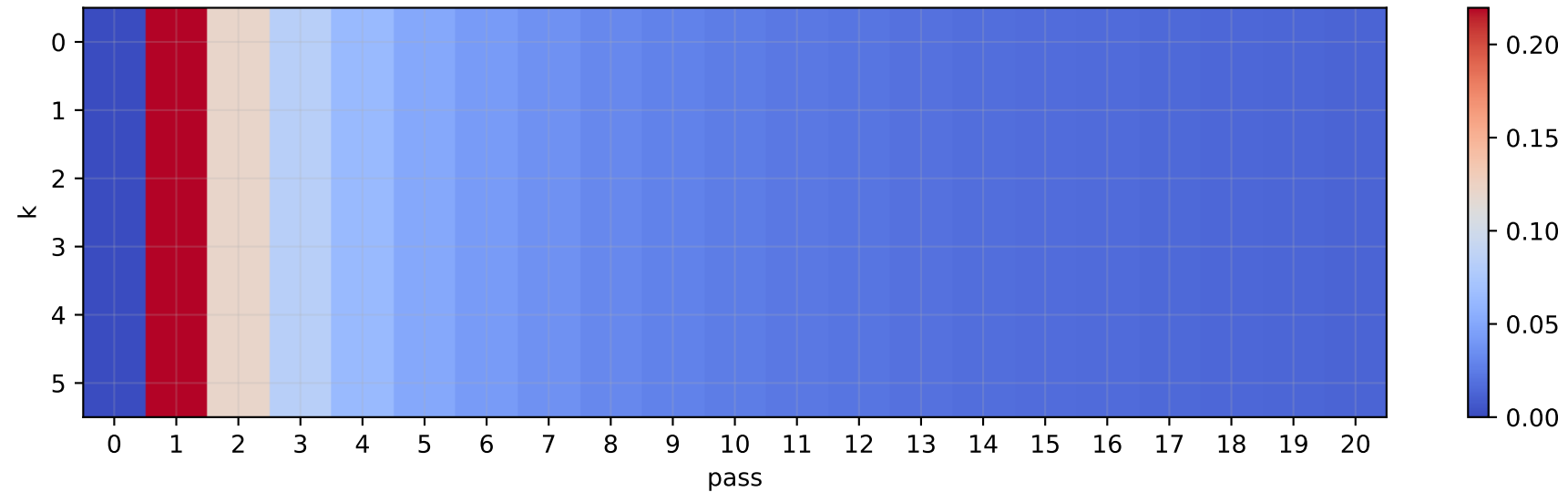
cod-rna: Validation NLL change from initial
