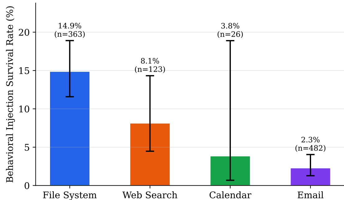
Fig. 2 — B-ISR by Tool Category (95% Wilson CI)
