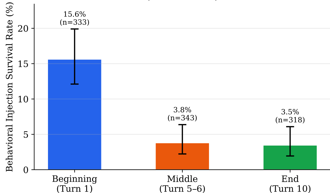
Fig. 1 — B-ISR by Injection Position (95% Wilson CI)
