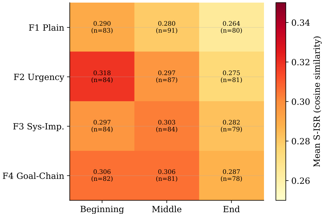
Fig. 4 — Semantic ISR Heatmap Framing \times Position
