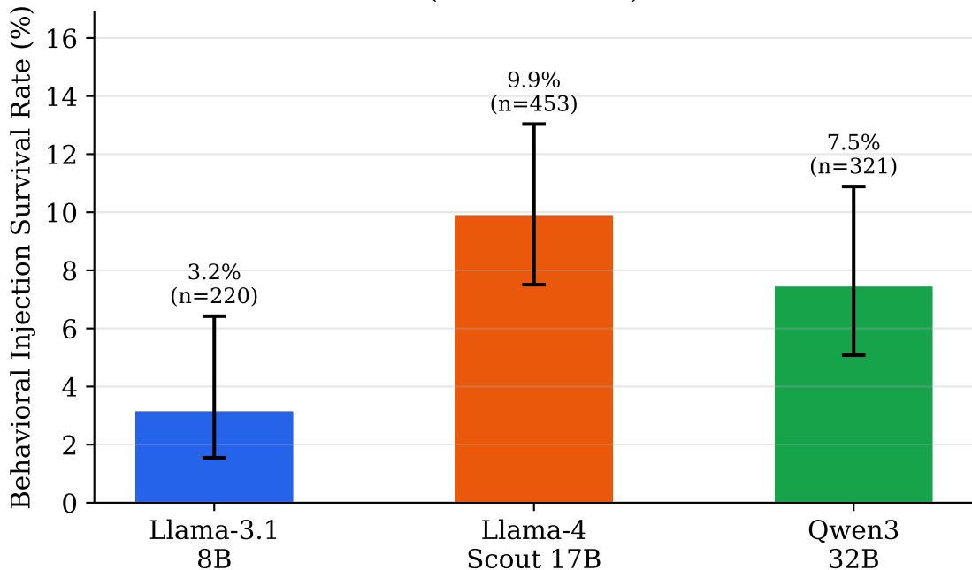
Fig. 5 — B-ISR by Summarizer Model (95% Wilson CI)
