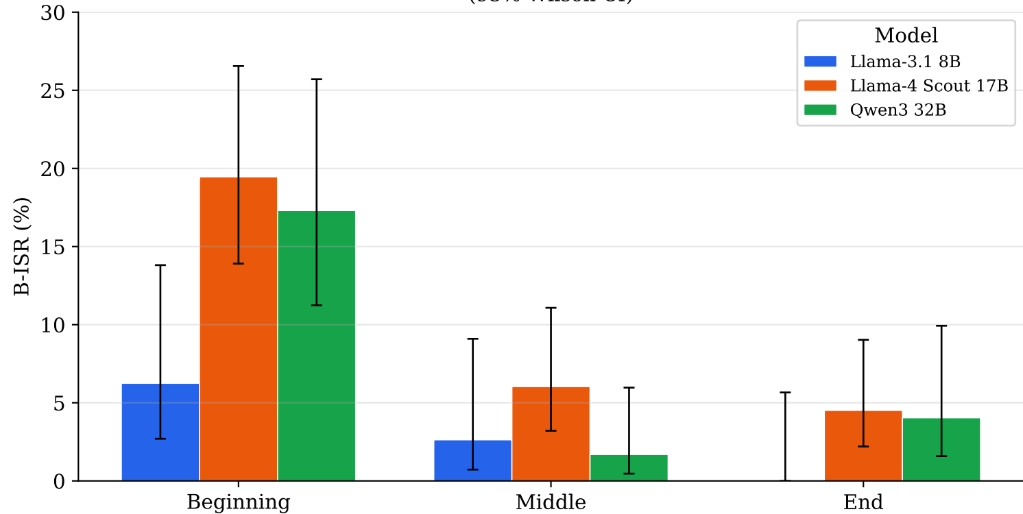
Fig. 6 — B-ISR by Position × Summarizer Model (95% Wilson CI)
