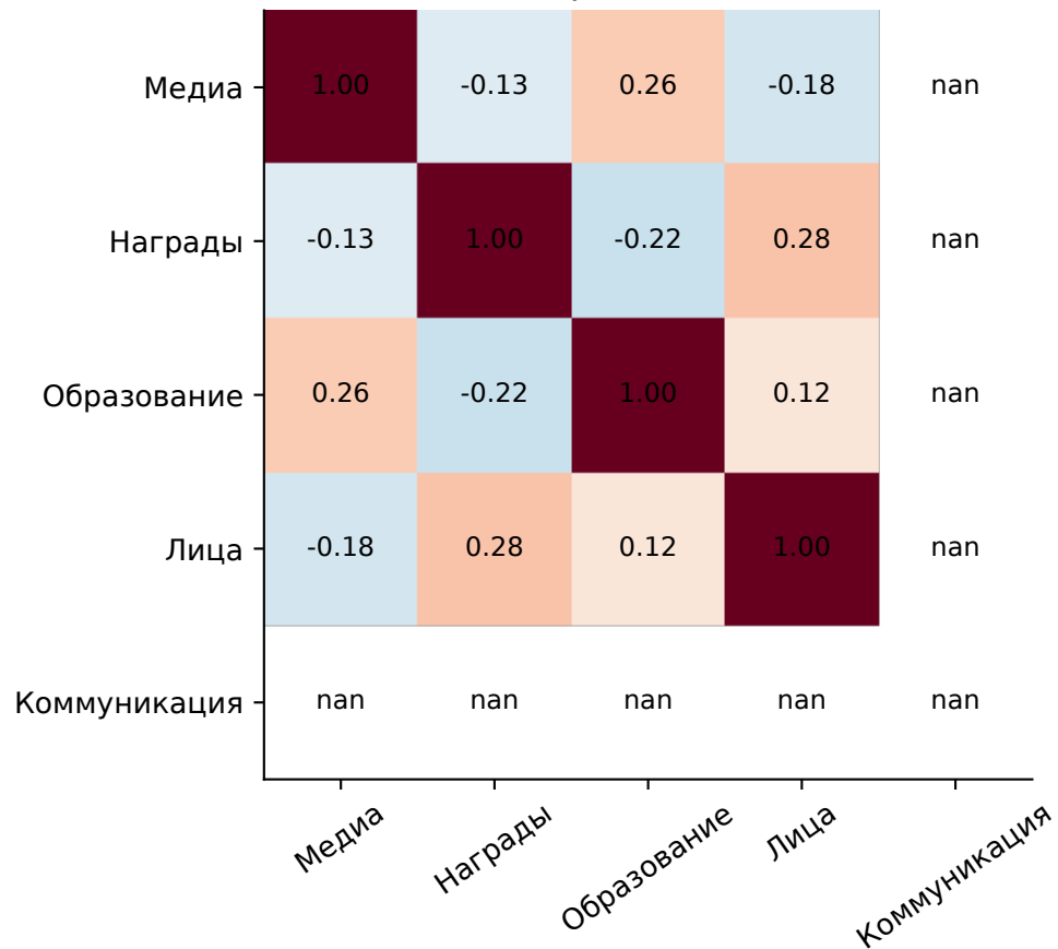
CEO: Spearman, n=28
