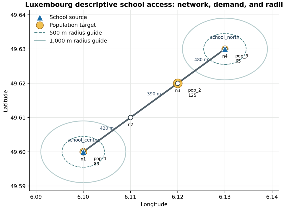
Figure 2: Illustrative Luxembourg data objects used in the notebook: a small road network with edge lengths, two school source points, three population target points, and schematic 500 m and 1,000 m radius guides. The country-scale run uses the same object contracts after extracting OSM schools and WorldPop target cells; the radius guides are visual aids, while coverage is computed from network distances.
