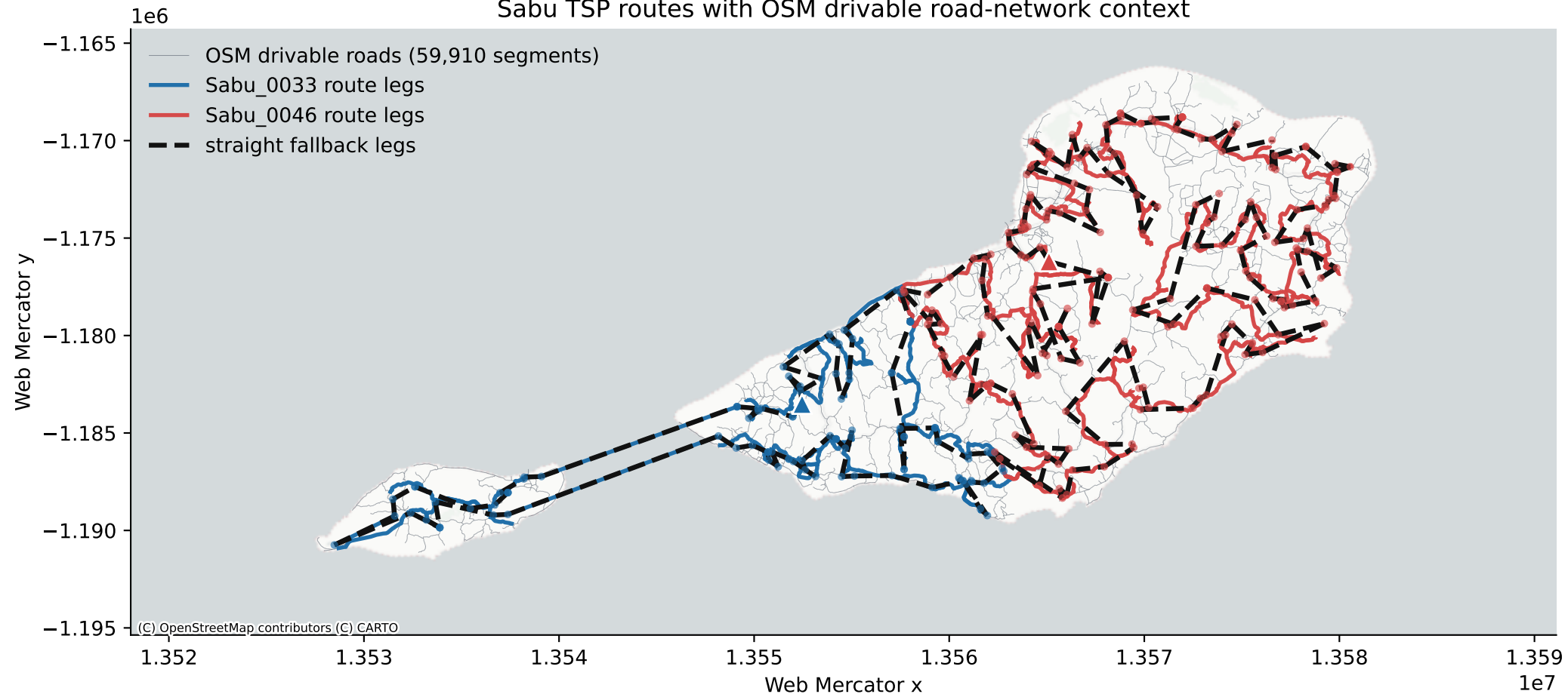
Sabu TSP routes with OSM drivable road-network context
