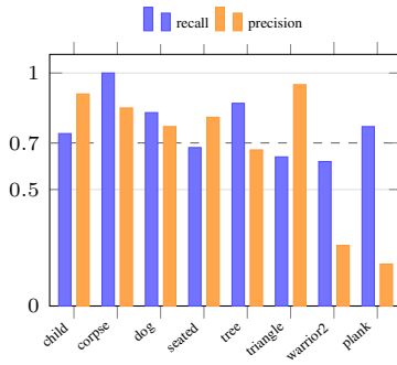
(b) ST-GCN, held-out videos, per pose
