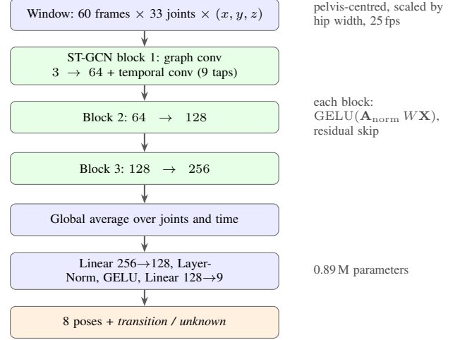
(b) The ST-GCN sequence model ("flow check").
