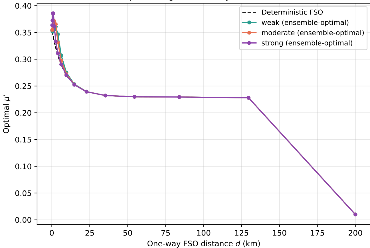
Optimal signal intensity vs distance
