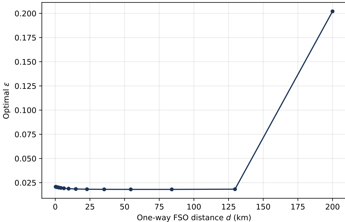
Deterministic FSO: optimal sending probability vs distance
