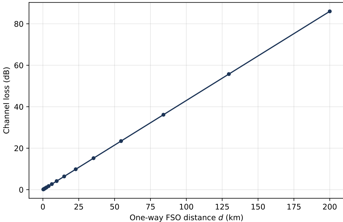
Deterministic FSO: channel loss vs distance
