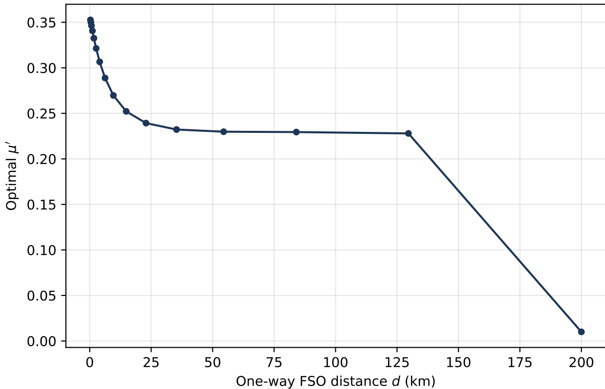
Deterministic FSO: optimal signal intensity vs distance
