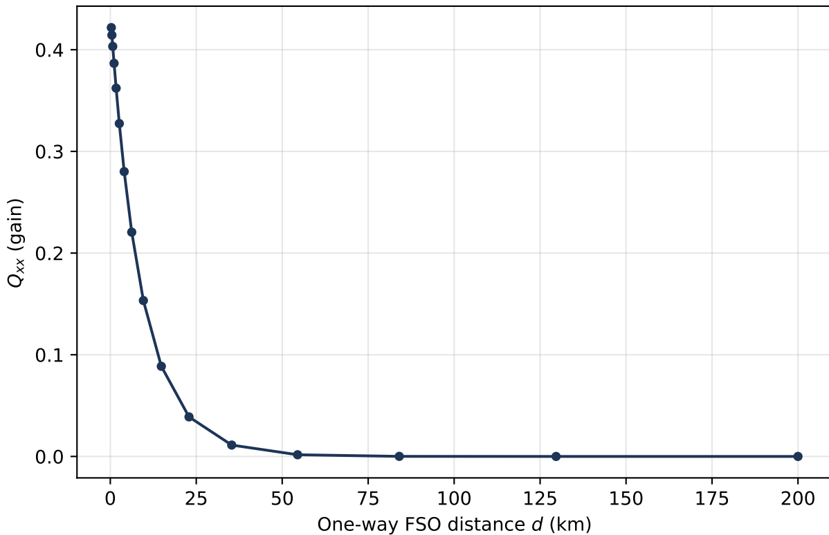
Deterministic FSO: Q_{xx} vs distance
