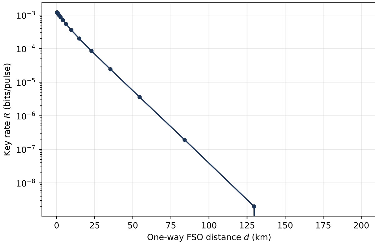
Deterministic FSO: SKR vs distance
