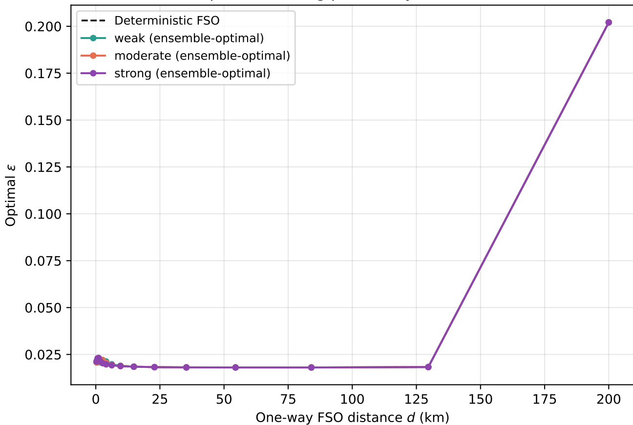
Optimal sending probability vs distance
