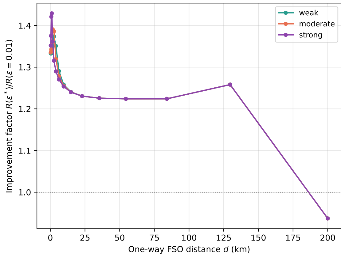
SKR improvement from optimising \varepsilon (mild baseline \varepsilon = 0.01 )
