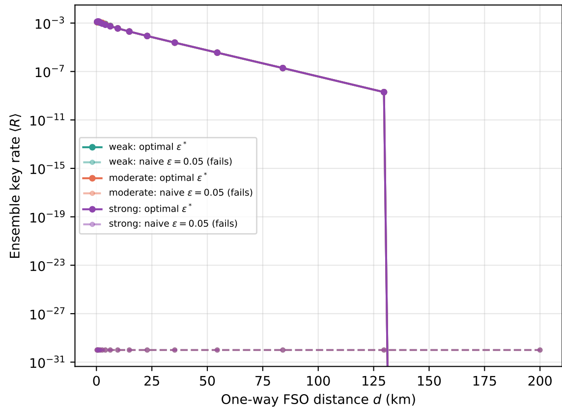
Optimal \varepsilon^* vs a poorly-chosen \varepsilon = 0.05
