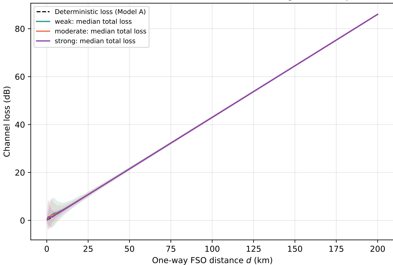
Channel loss: deterministic + Gamma-Gamma fading (5th-95th pct band)
