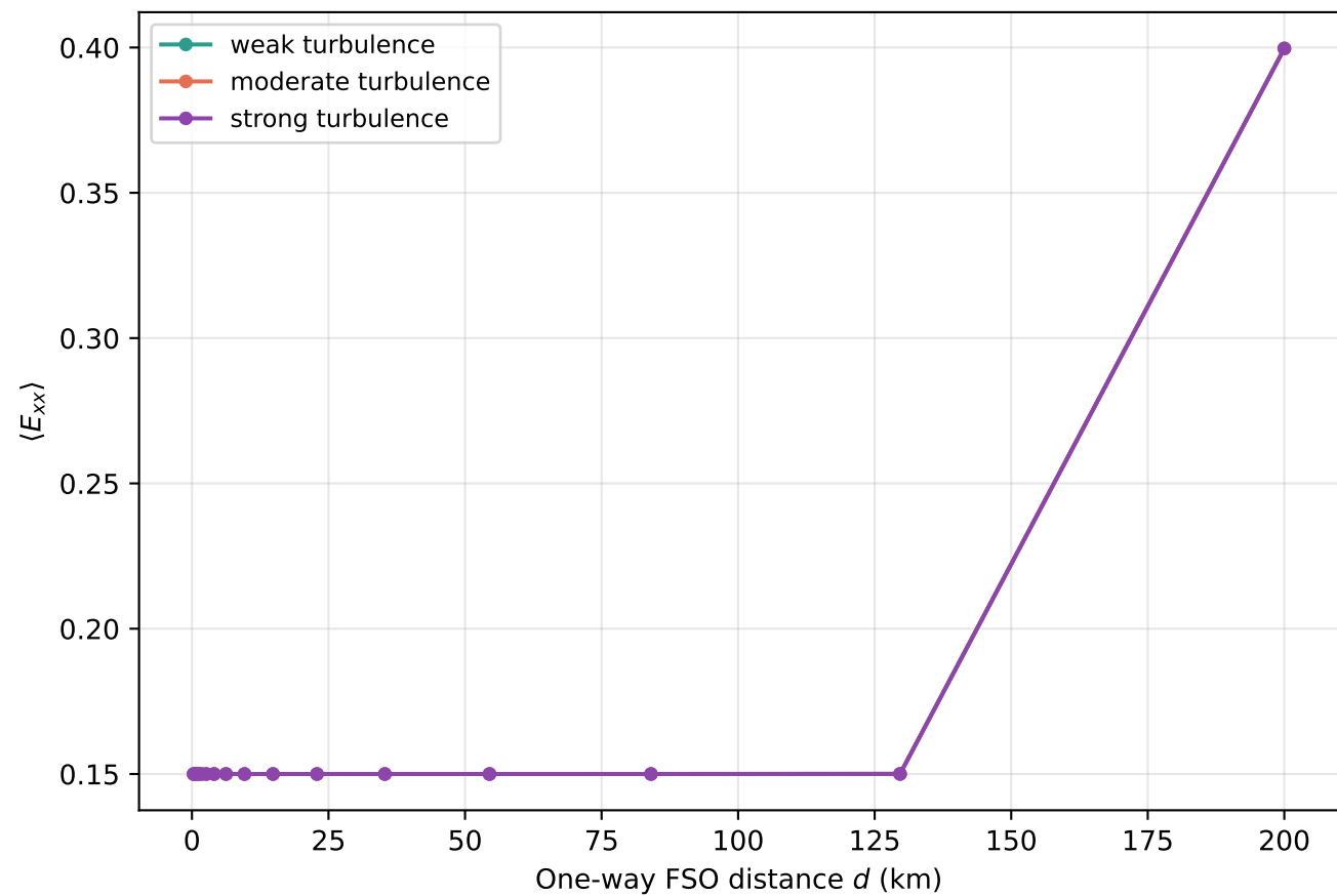
Gamma-Gamma: E_{xx} vs distance
