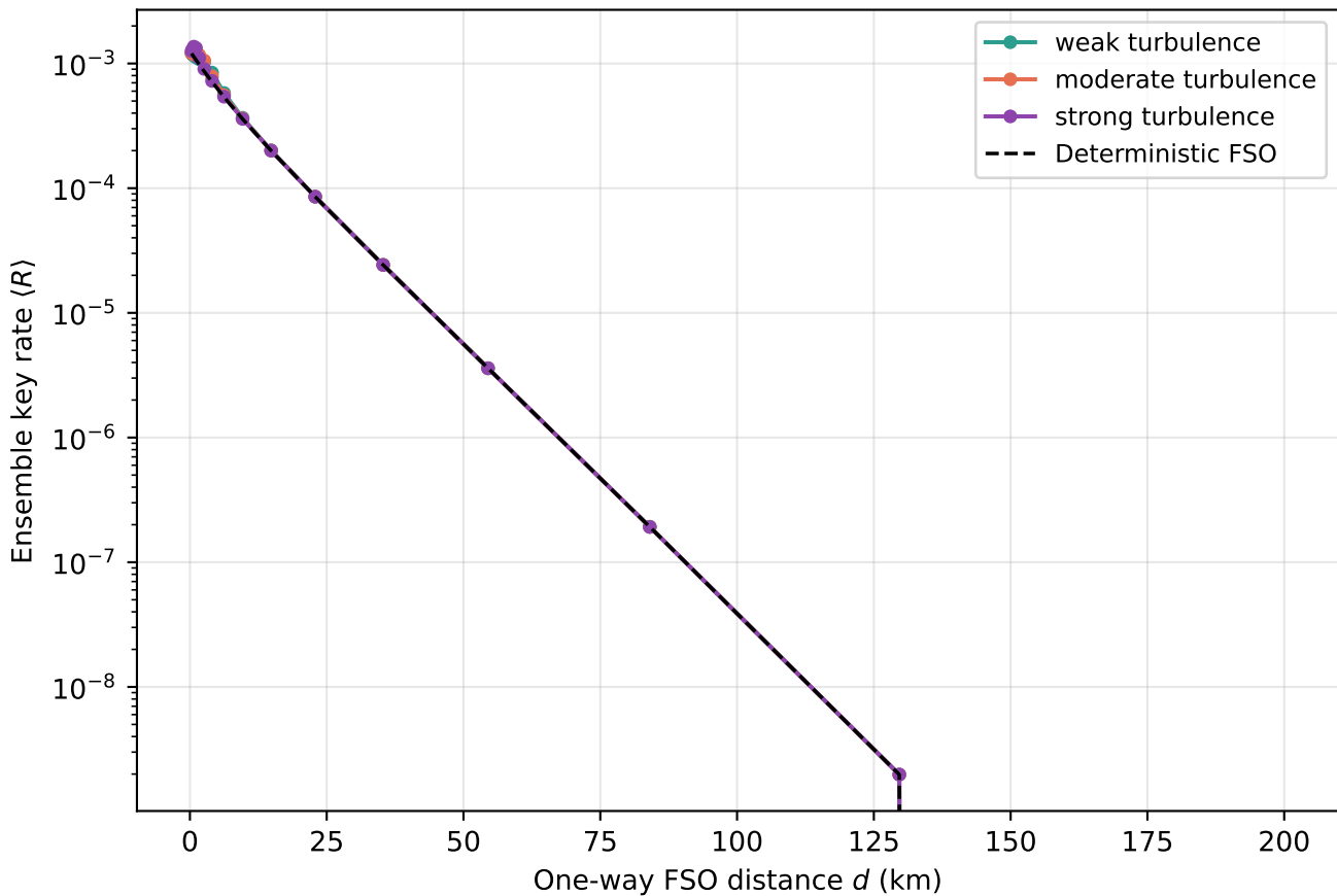
Gamma-Gamma: SKR vs distance (Monte Carlo)
