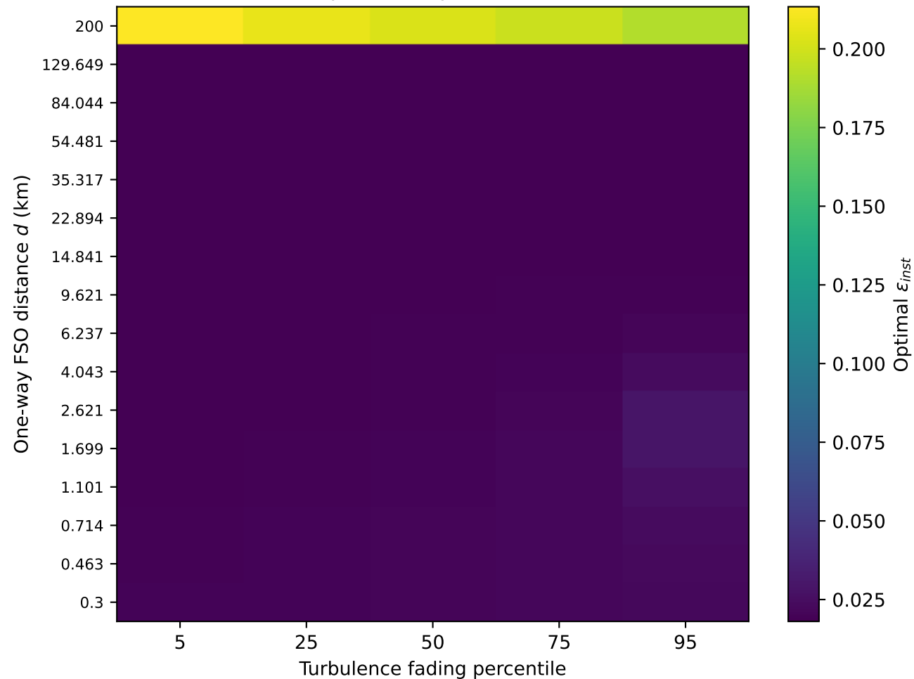
Instantaneous epsilon map (moderate turbulence)
