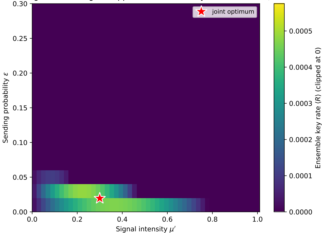
Joint optimisation landscape (d=6.0 km) (negative-rate region clipped to 0 for visibility; \varepsilon axis zoomed)
