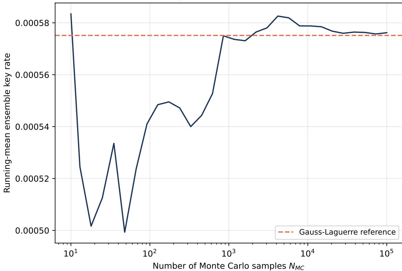
Monte Carlo convergence (d=6.0 km, moderate turbulence)
