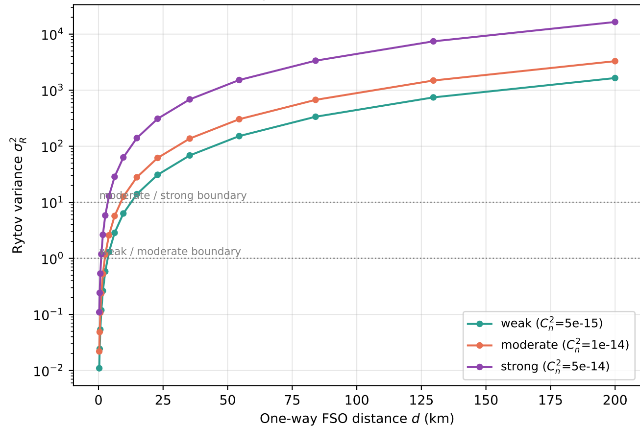
Rytov variance vs distance
