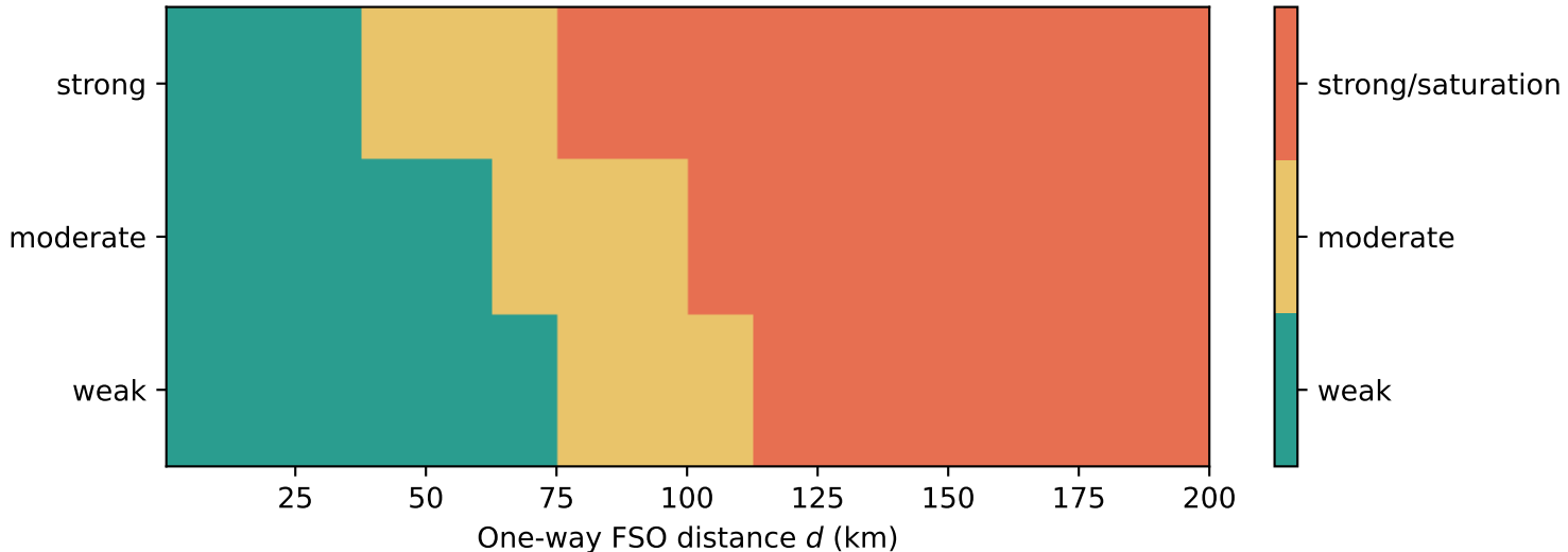
Turbulence regime map (Gamma-Gamma validity classification)
