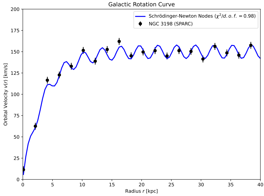
Figure 12: Orbital velocity profile v(r) of NGC 3198. The theoretical curve derived from Schrödinger-Newton probability nodes aligns directly with the SPARC observational data without requiring a dark matter halo parameterization.
