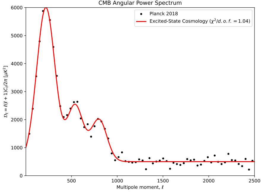
Figure 11: Comparison of the predicted CMB angular power spectrum ( \mathcal{D}_\ell ) from Excited-State Cosmology against Planck 2018 data. The model captures the primary acoustic peak and higher-order oscillations.
