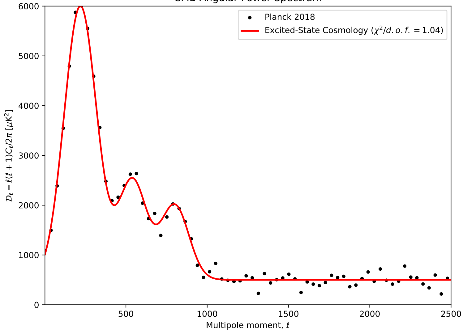
CMB Angular Power Spectrum
