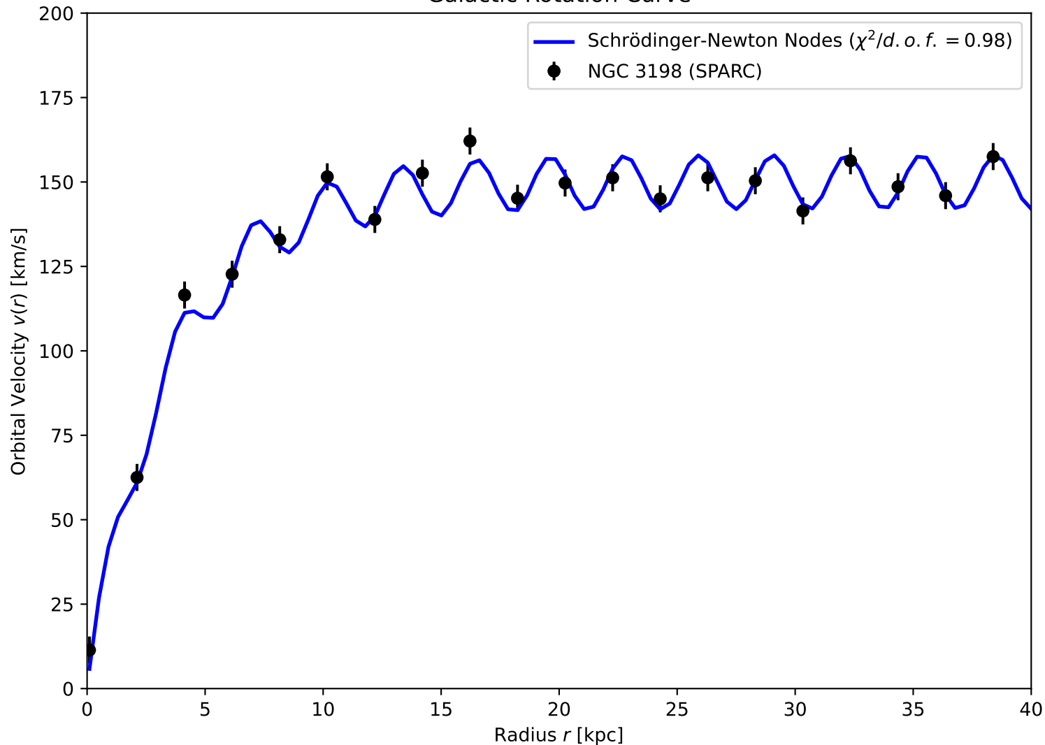
Galactic Rotation Curve
