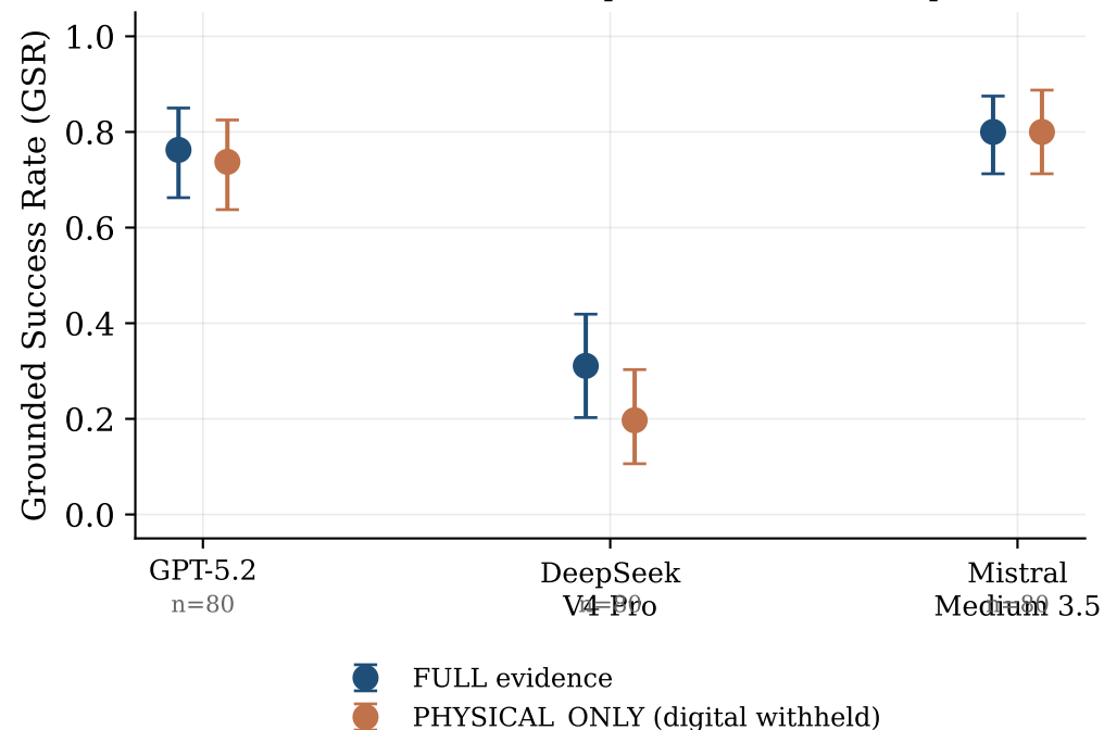
(a) GSR, FULL vs digital-withheld (n=80 worlds) error bars = bootstrap 95% CI -- all overlap
