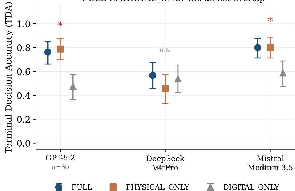
(b) TDA across all regimes (n=80 worlds) * = FULL vs DIGITAL_ONLY CIs do not overlap
