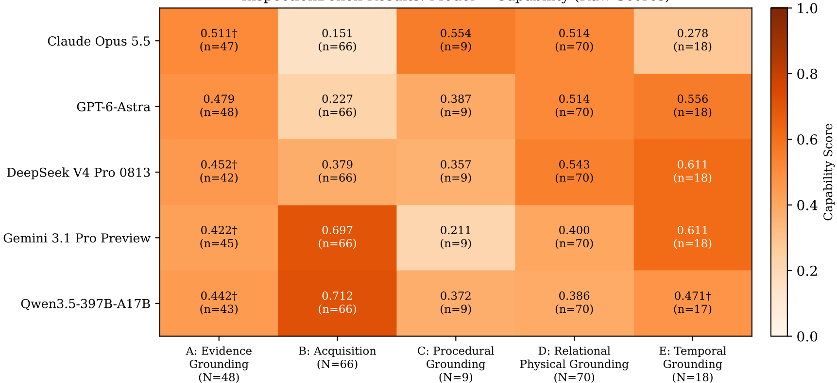
InspectionBench Results: Model × Capability (Raw Scores)
