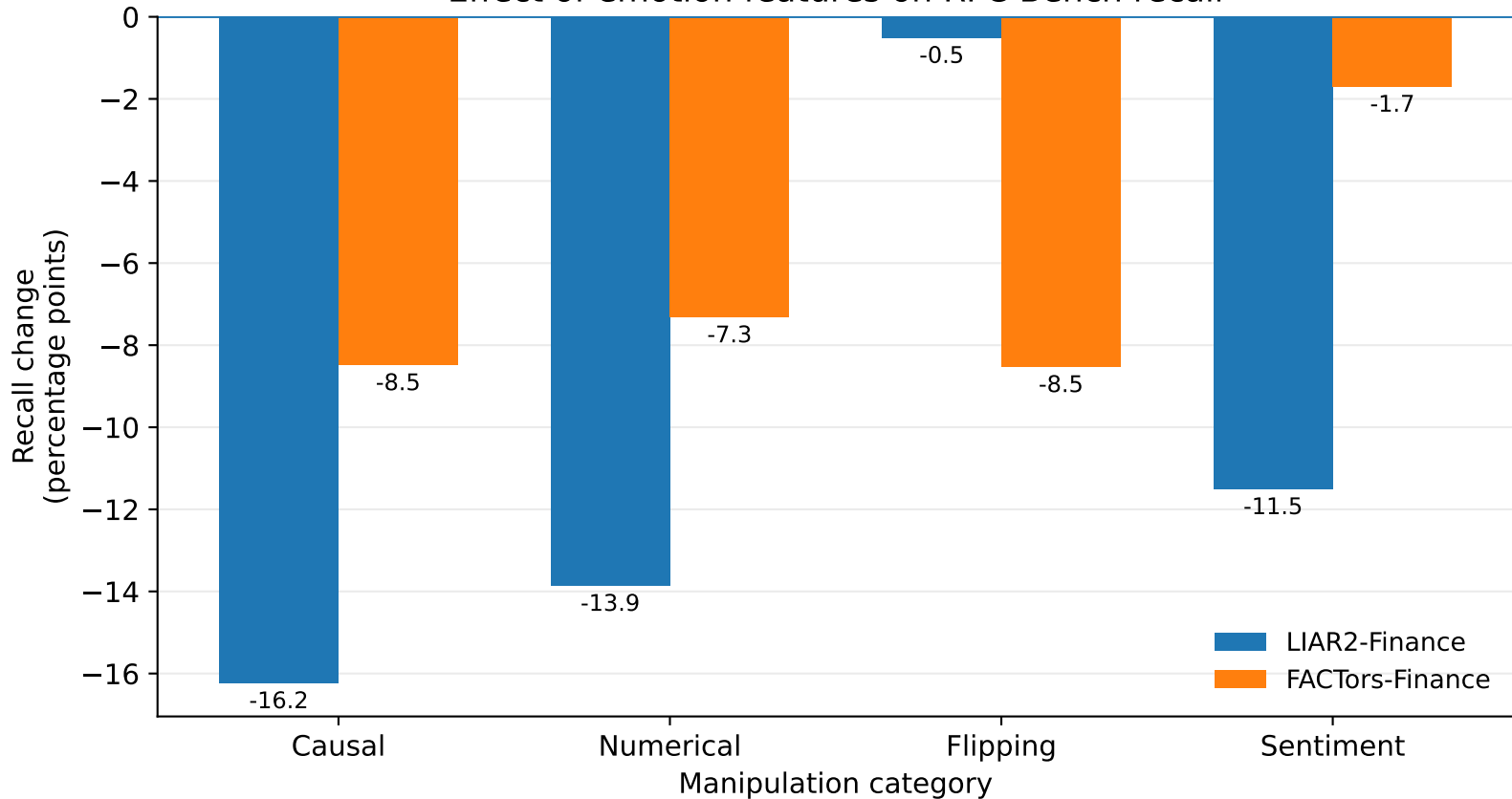
Effect of emotion features on RFC-Bench recall
