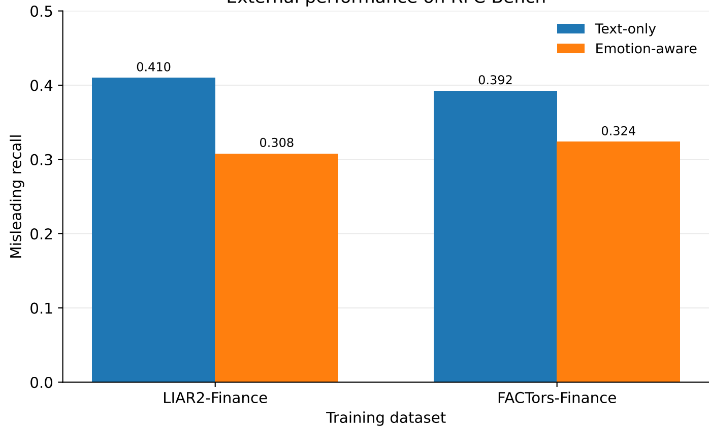
External performance on RFC-Bench
