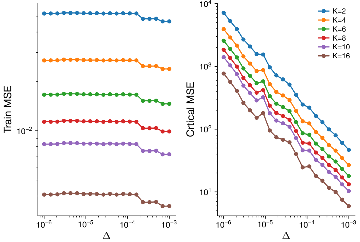
Error vs \Delta ( \nu=0.75 )
