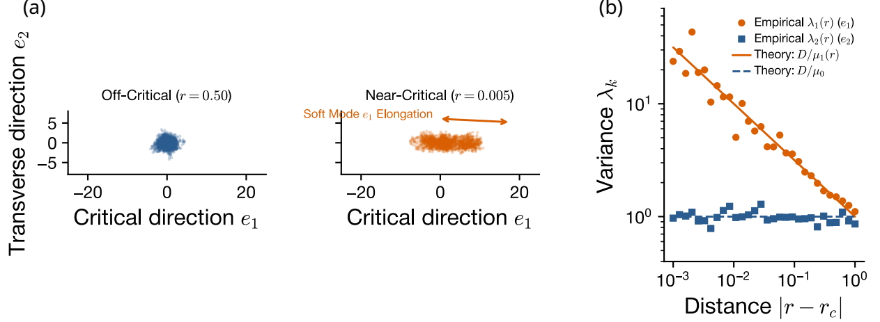
Figure 1: (a) Dynamical origin of spatial anisotropy. Steady-state sample distributions in state space generated by the multidimensional Langevin process off-criticality ( r = 0.50 , left) and near-criticality ( r = 0.005 , right). As the control parameter r \rightarrow r_c , the restoring force along the critical mode vanishes ( \mu_1(r) \rightarrow 0 ), driving anisotropic fluctuation growth and severe elongation along the soft mode direction e_1 , while fluctuations along the transverse direction e_2 remain tightly bounded. Shaded regions depict the 2\sigma spatial covariance ellipses. (b) Empirical covariance spectrum. Eigenvalues of the empirical covariance matrix \Sigma plotted against the distance to criticality |r - r_c| . The dominant eigenvalue \lambda_1(r) diverges as D/\mu_1(r) \sim |r - r_c|^{-\nu} (with \nu = 0.50 ), whereas transverse eigenvalues \lambda_{k \geq 2} remain stationary ( D/\mu_0 = O(1) ), confirming the dynamical emergence of a low-dimensional critical manifold.
