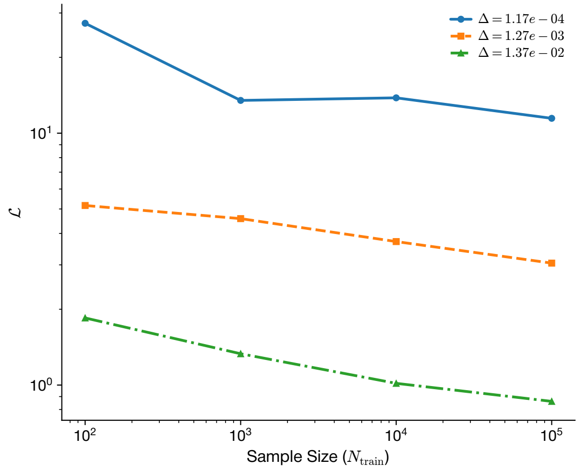
Critical MSE vs N_{\text{train}}
