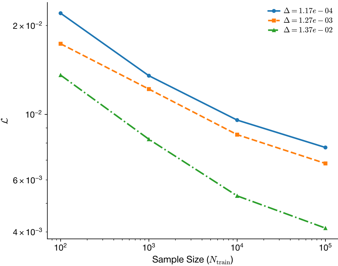
Train MSE vs N_{\text{train}}
