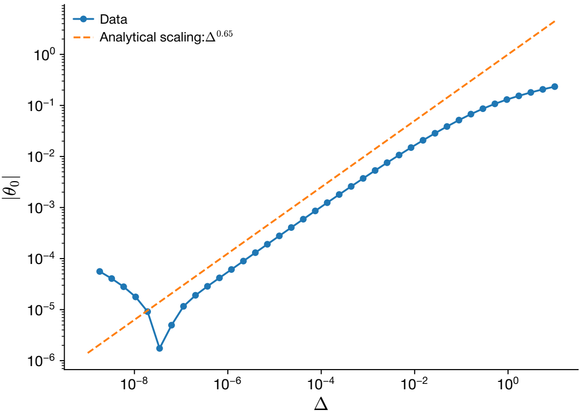
\theta vs \Delta , \nu = 0.35
