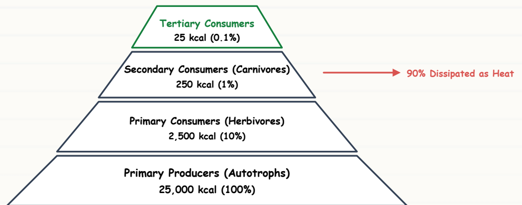
Figure 1.2: Unidirectional Energy Dissipation Following Lindeman's 10% Law
