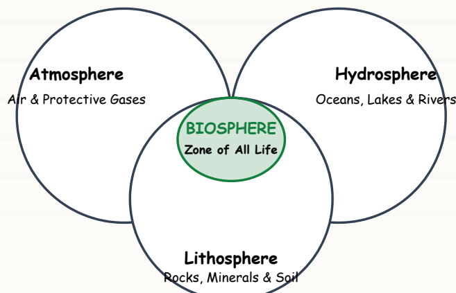
Figure 1.1: The Interlocking Spheres of Earth's Environment
