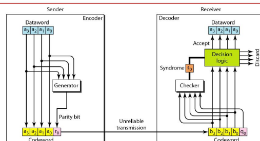
Figure 10.10 Encoder and decoder for simple parity-check code
